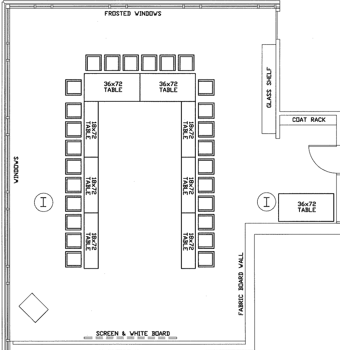
25' x 36' FORD ROOM U-SHAPED LAYOUT
