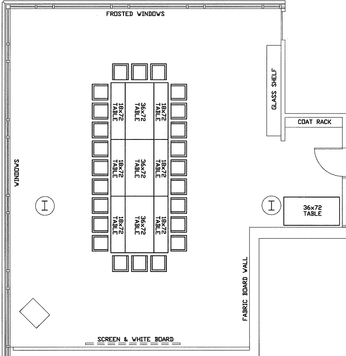
25' x 36' FORD ROOM CONFERENCE LAYOUT
